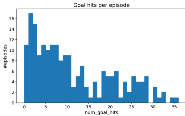
Fig. 15. Distribution of goal hits per episode for the Shadow Hand.
