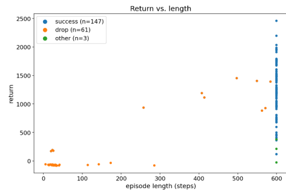
Fig. 8. Return as a function of episode length. Instances where the cube converged close to the target orientation but failed to complete the reorientation task are highlighted in green.
