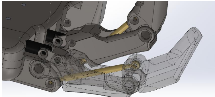
Fig. 1. teal linkages (yellow) connecting the distant phalanx with the driven middle phalanx.
