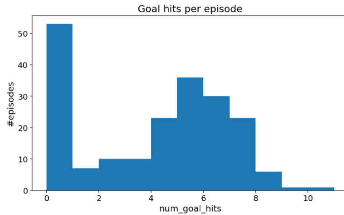
Fig. 5. Distribution of goal hits per episode for the 7-DoF Bionic Hand with extended supination.
