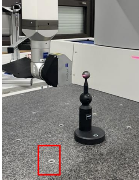
Fig. 5. Laser sensor qualification [11]
