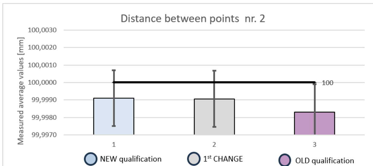
Fig. 8. Contact measurement – distance between points
