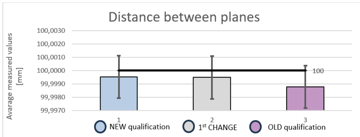
Fig. 7. Contact measurement – distance between planes
