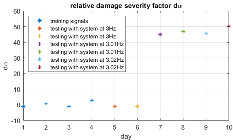
Fig. 7. Relative damage severity factor behaviour
