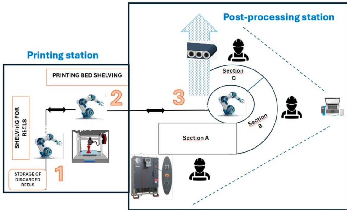
Fig. 1. Layout production cell
