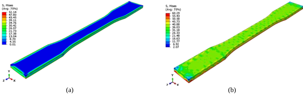
Fig. 3. Residual stresses of test specimen (a) at the end of extrusion, (b) at the end of cooling, where S is in (MPa).
