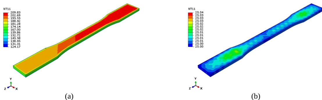
Fig. 2. Temperature distribution (a) temperature distribution of test specimen at the end of extrusion, (b) at the end of cooling, where NT11 represents the nodal temperature (°C).
