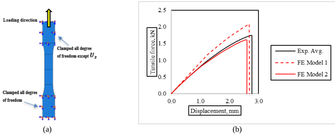
Fig. 4. (a) Tensile test simulation setup, (b) Force-displacement curve where Exp. Avg. Represents the average typical values obtained from the physical tests [15]. FE Model 1, FE Model 2 represent the first and second tensile test simulations respectively.
