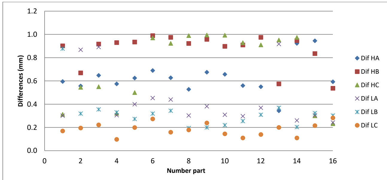
Fig. 5. Calculated deviations from nominal dimensions
