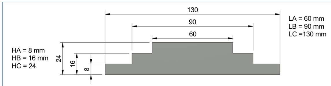
Fig. 1. Specimens dimensions.
