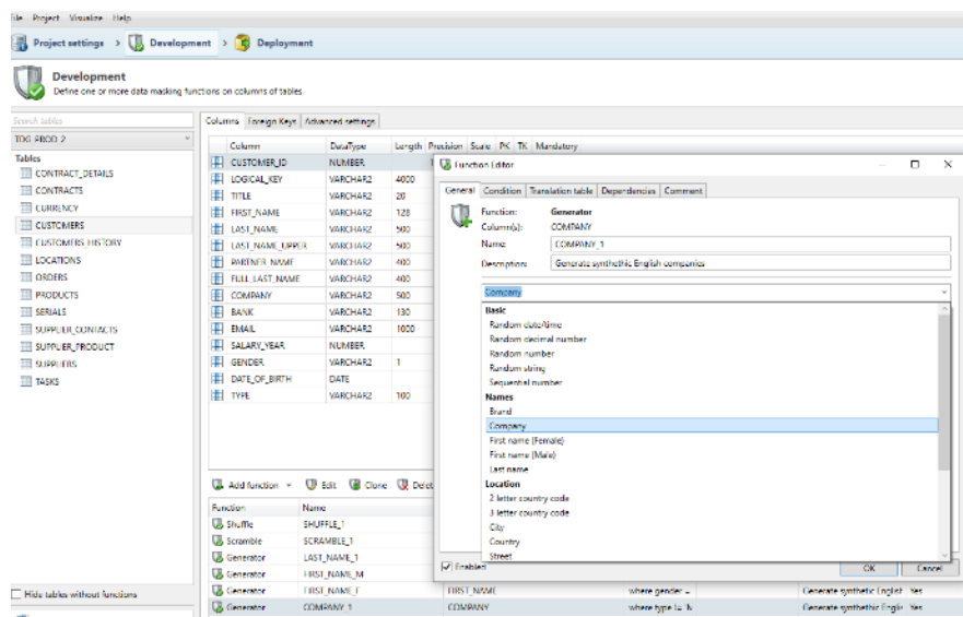
Fig. 1. DATPROF tool interface (picture from: https://www.datprof.com/ . Accessed on 07.07.2024.)
