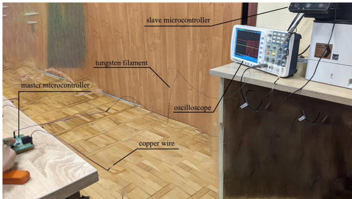
Fig. 2. Experimental setup
