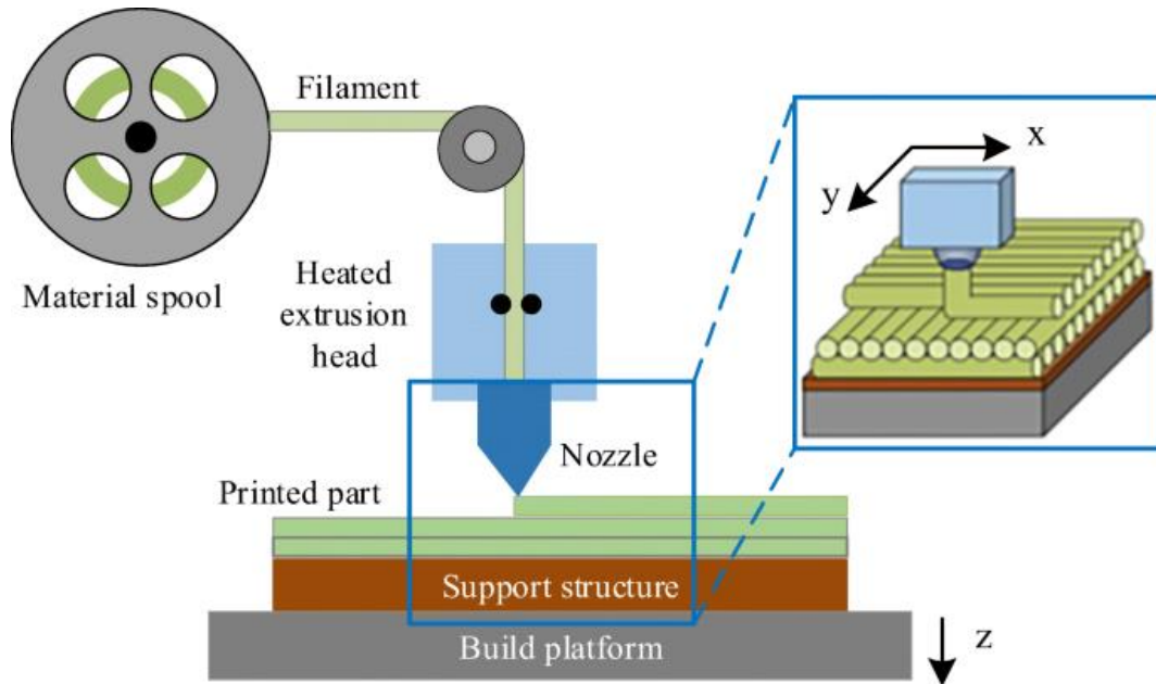
Fig. 1. FDM 3D printing technology process [5]
