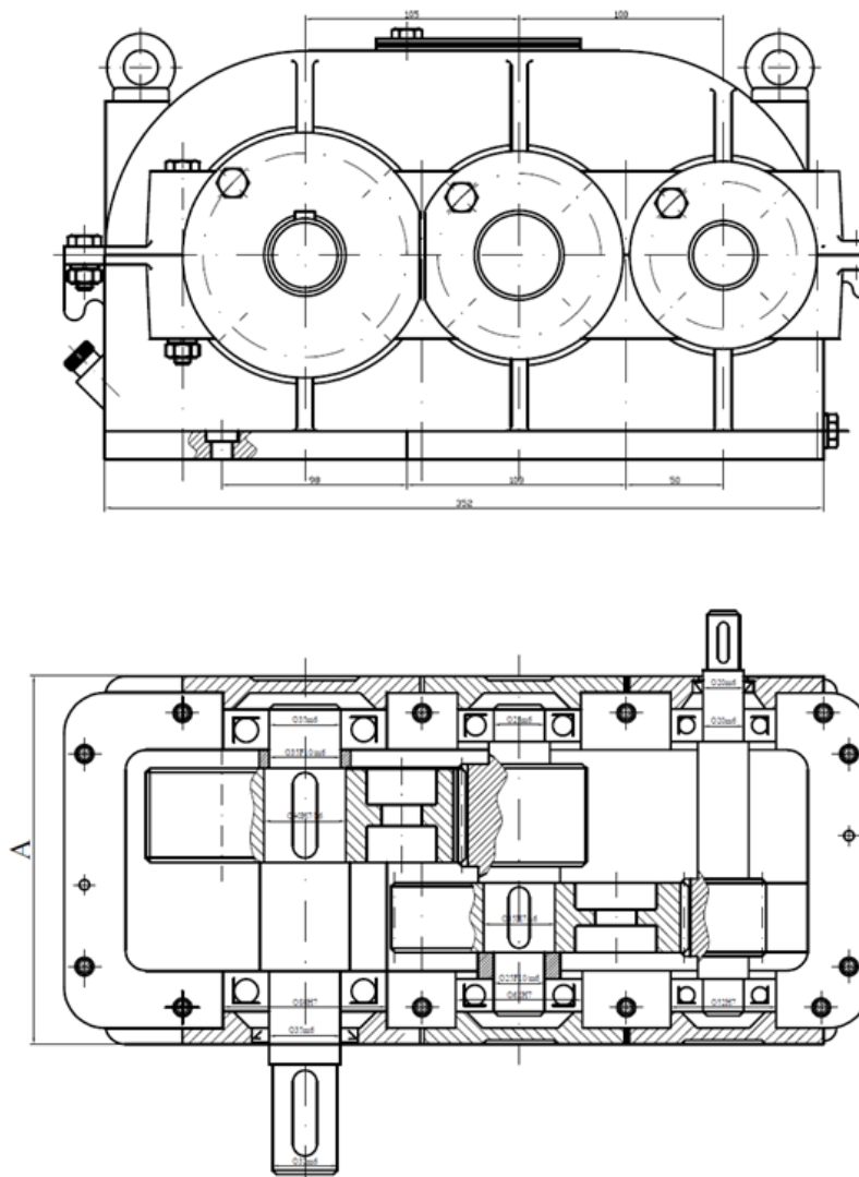
Fig. 1. Model of driving mechanism, [15]
