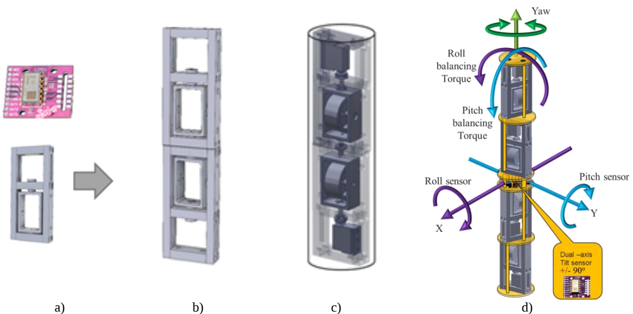
Fig. 7. Dual-Axis tilt sensor + evolution of Gimbals & Frame + future construction
