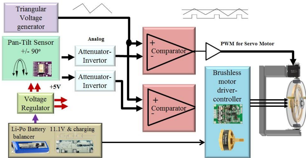
Fig. 8. Functional Diagram of the CMG Analog control
