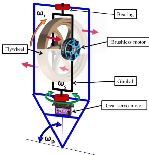
Fig. 2. Scheme of parrying disturbances
