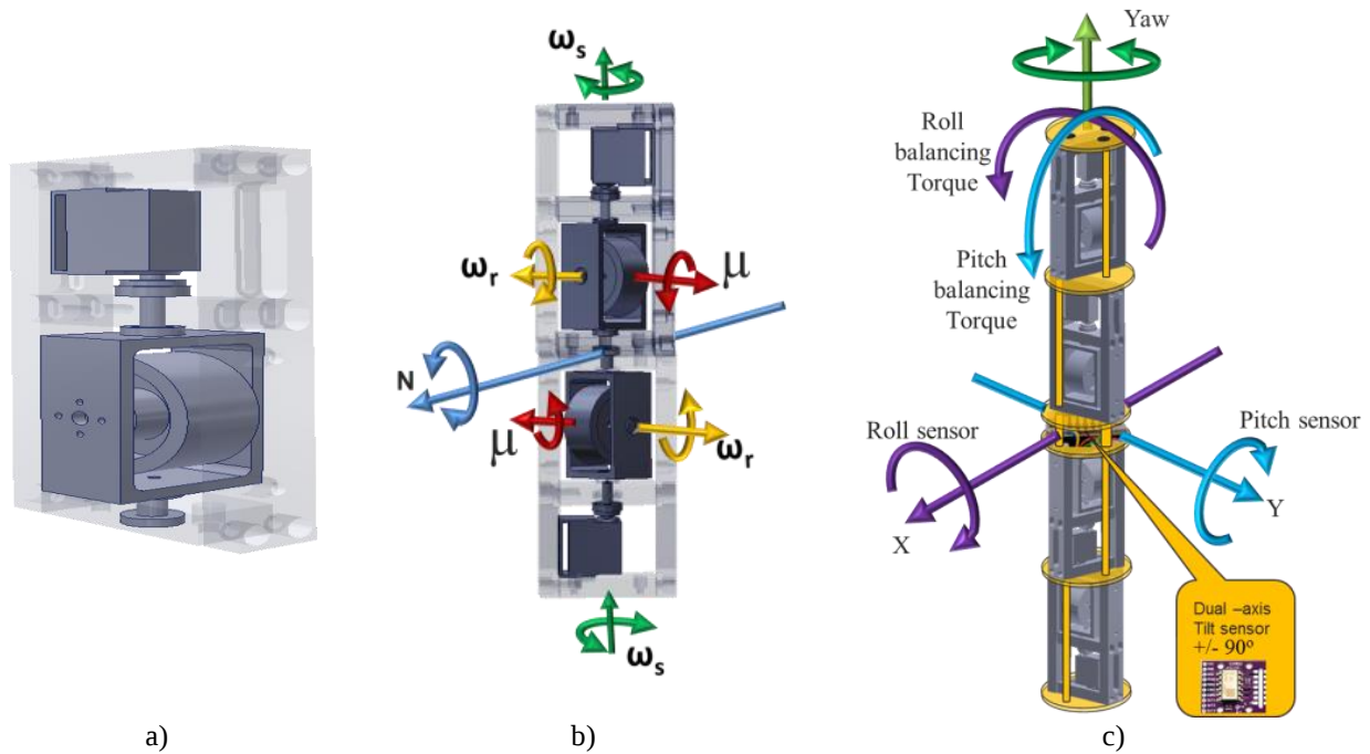
Fig.4. 3D model of the CMG self-balancing robotic spine
