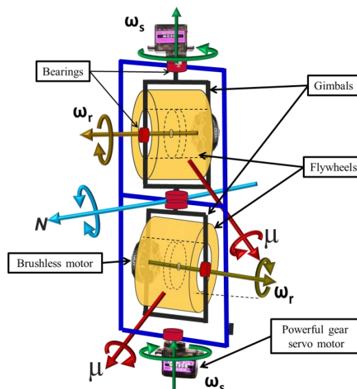
Fig. 1. A section of the robotic spine
