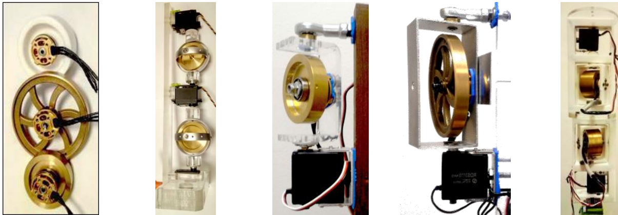
Fig. 5. Evolution of the attempts of CMG prototyping
