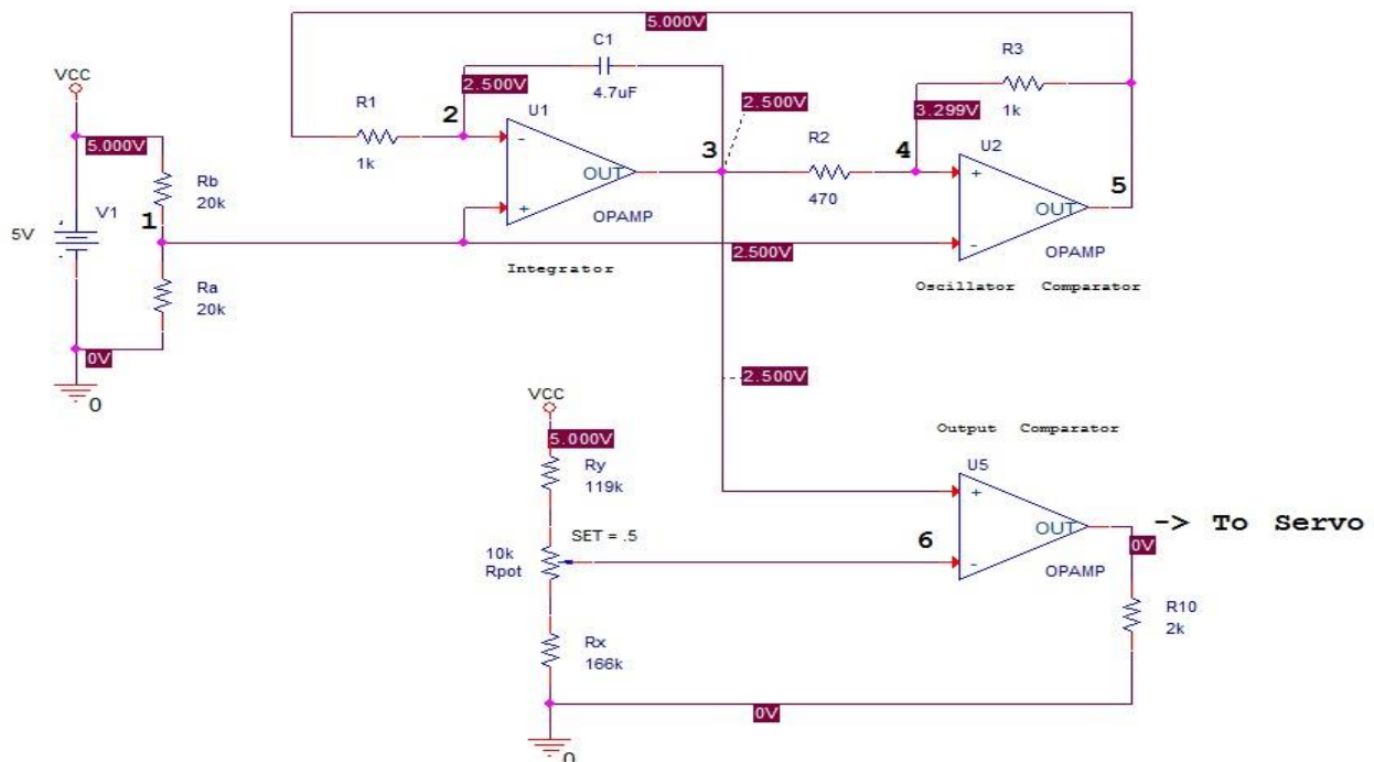
Fig. 9. Electrical diagram of the CMG Analog control
