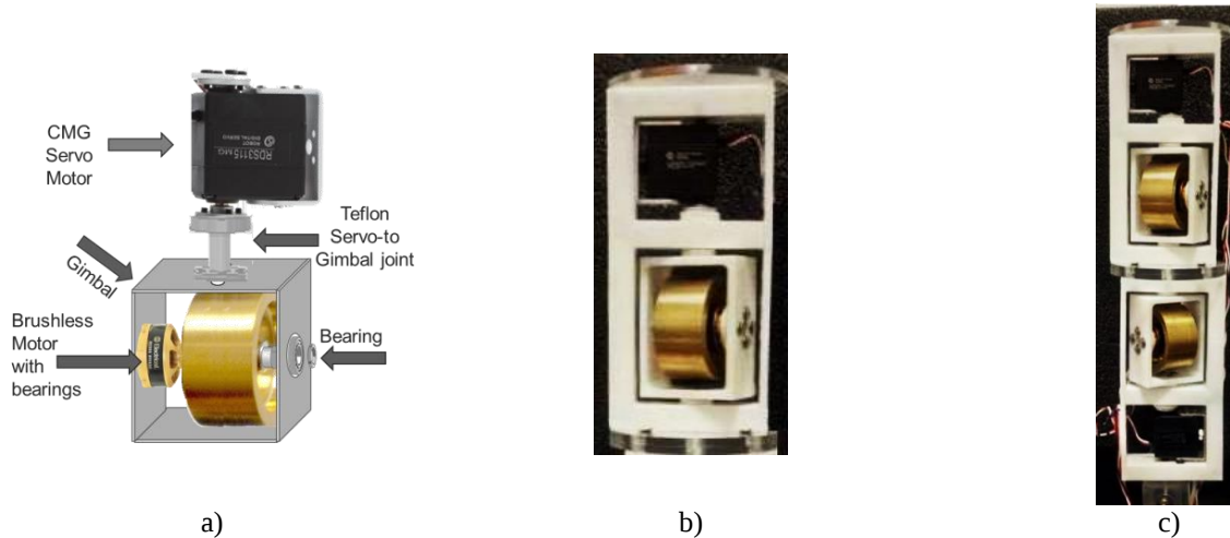
Fig. 6. Brushless motor and CMG module
