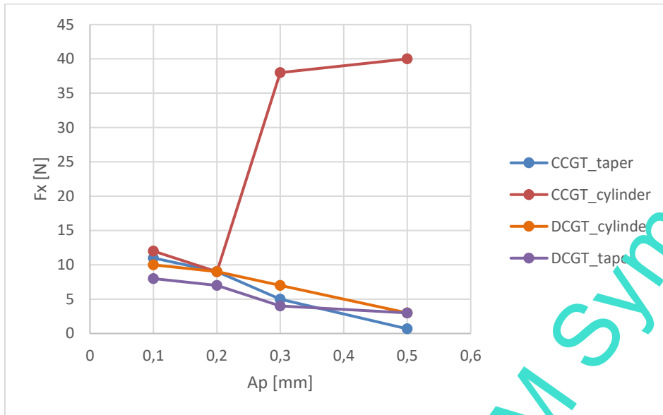
Fig. 8. Dependence between DOC and cutting force in the X axis direction
