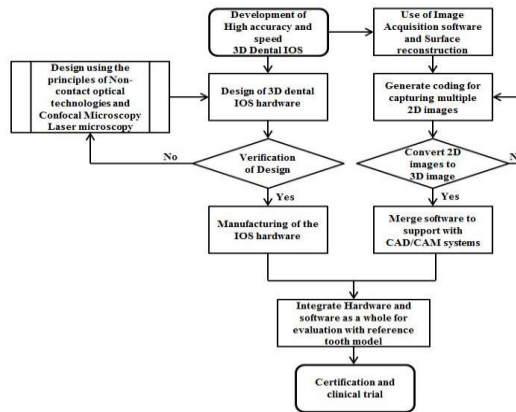
Fig.3. Schematic procedure to develop 3D dental IOS for high accuracy and speed.
