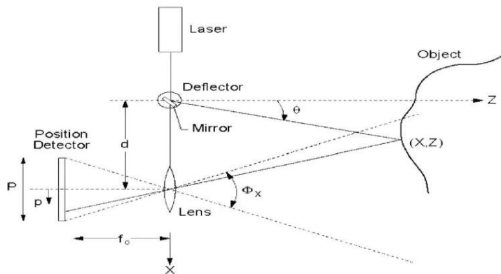
Fig.6 2D active triangulation method [12].
