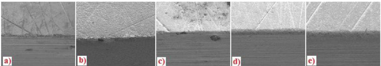
Fig. 5. Cutting edge prepared by: a) grinding, b) laser technology to edge radius 5 \mu\text{m} and drag finishing to edge radius c) 5 \mu\text{m} , d) 10 \mu\text{m} and e) 15 \mu\text{m} (500x zoom).
