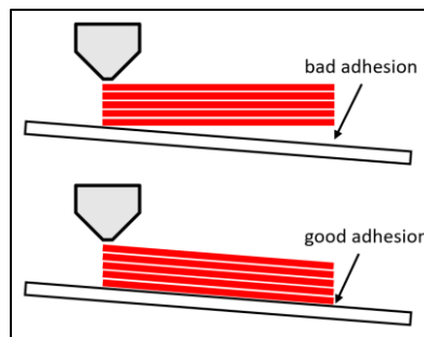
Fig. 5. Print with no bed leveling (top) and with bed leveling (bottom) (modified adopted from: [7])
