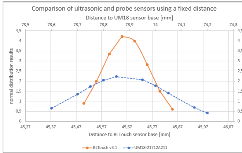
Fig. 7. Comparison of ultrasonic and probe sensors using a normal distribution
