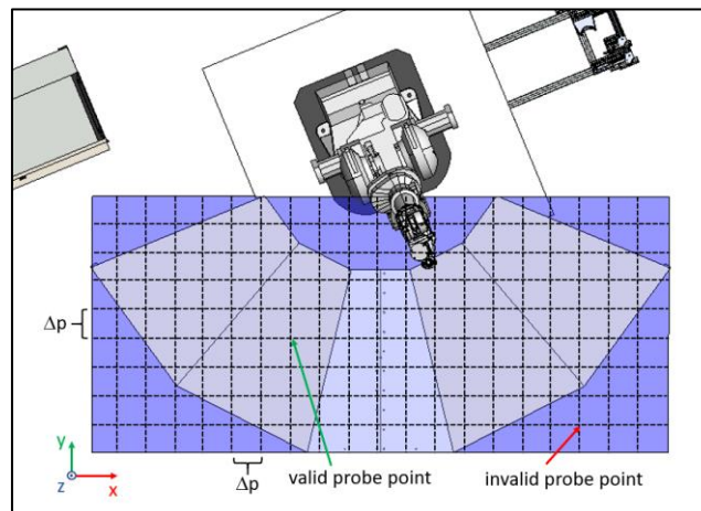
Fig. 8. Probing grid algorithm concept
