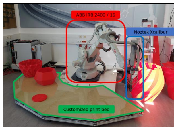
Fig. 1. Robotic system used for 3D-printing, positioned in the Digital Factory of the UAS Technikum Wien
