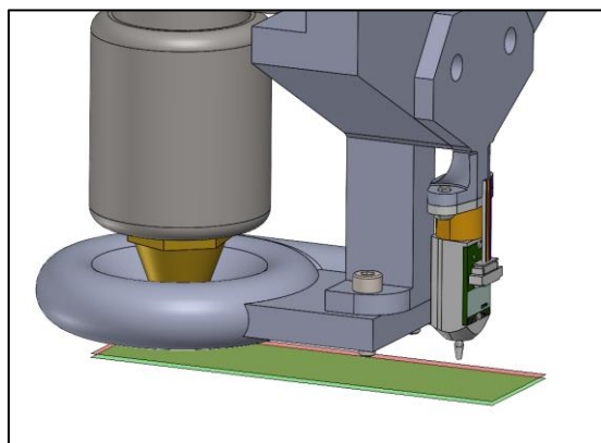
Fig. 9. Mounting point on the Noztek Xcalibur extruder using a 3D-printed plate
