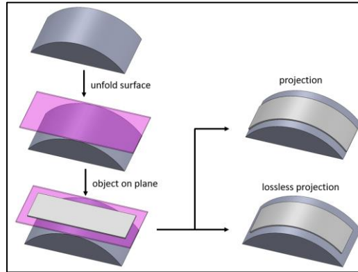
Fig. 6. Projection of a 2D object on a curved surface using normal projection and lossless projection (modified adopted from: [15])
