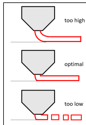
Fig. 4. Extruder nozzle distance to print bed (modified adopted from: [3])
