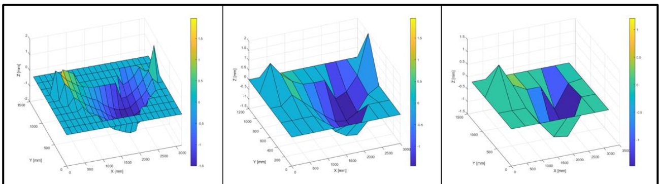
Fig. 12. Bed leveling results, 150 mm grid distance (left), 300 mm grid distance (middle), 450 mm grid distance (right)
