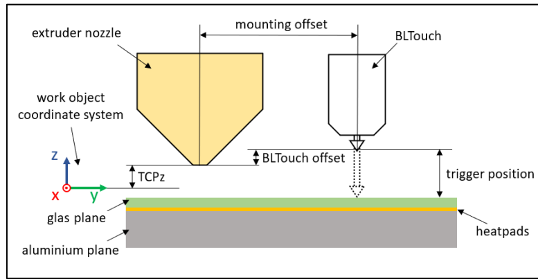
Fig. 10. Interpretation for the different offsets occurring with the mounting of the sensor
