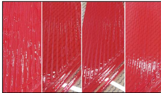
Fig. 15. Print quality with different extruder rotational speeds (from left to right: 1: 57 1/min [standard speed], 2: 30 1/min, 3: 20 1/min, 4: 15 1/min)
