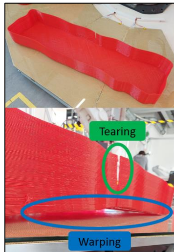
Fig. 3. Problems with current printing results on a relatively long object (top: aerial view of object; bottom: warping and tearing of the object)
