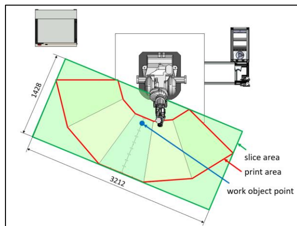
Fig. 2. Comparison of print area and slice area (top view of the system)
