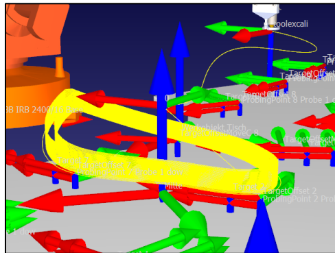
Fig. 13. Applying arbitrary probe results to the G-code in the simulation
