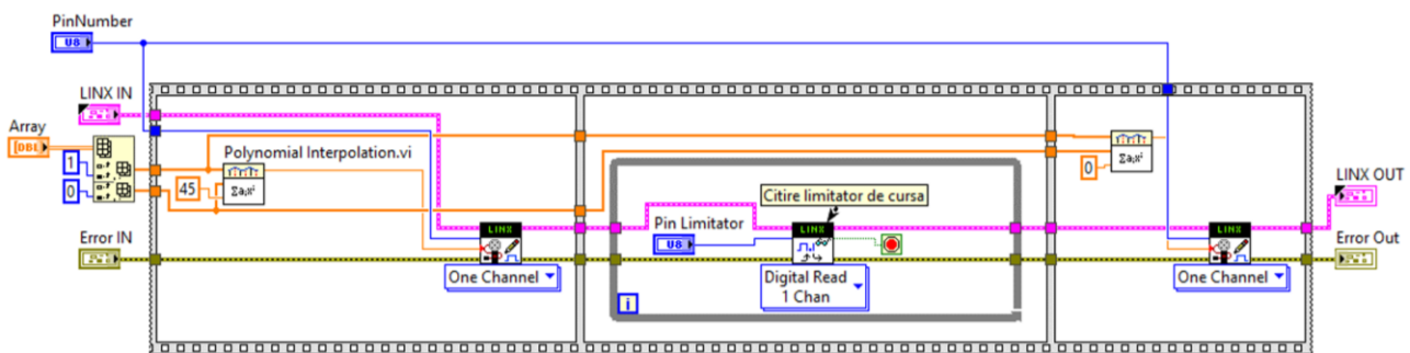
Fig. 7. Servomotor control
