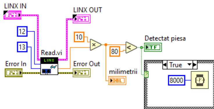
Fig. 6. Product detection algorithm
