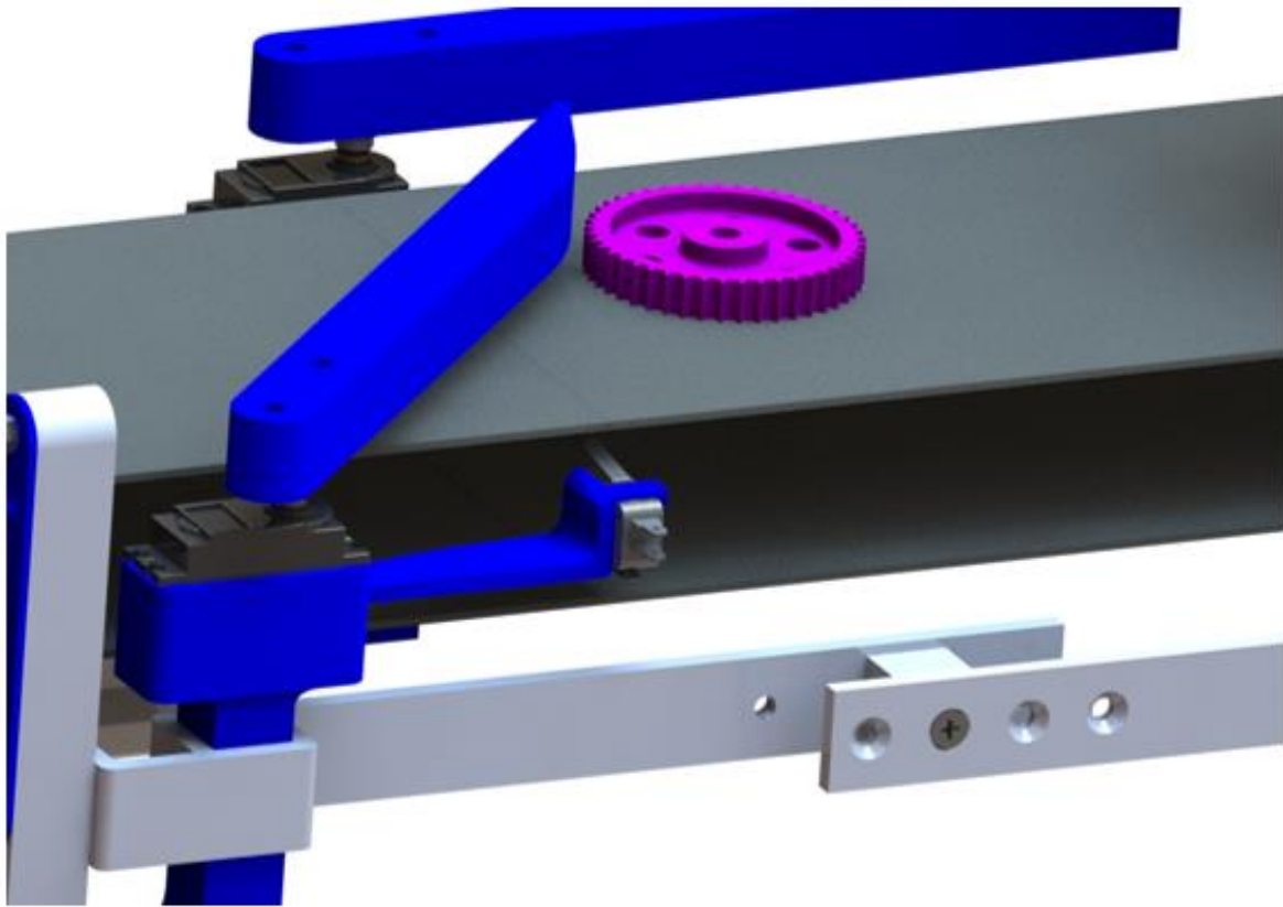
Fig. 2. Separation subsystem
