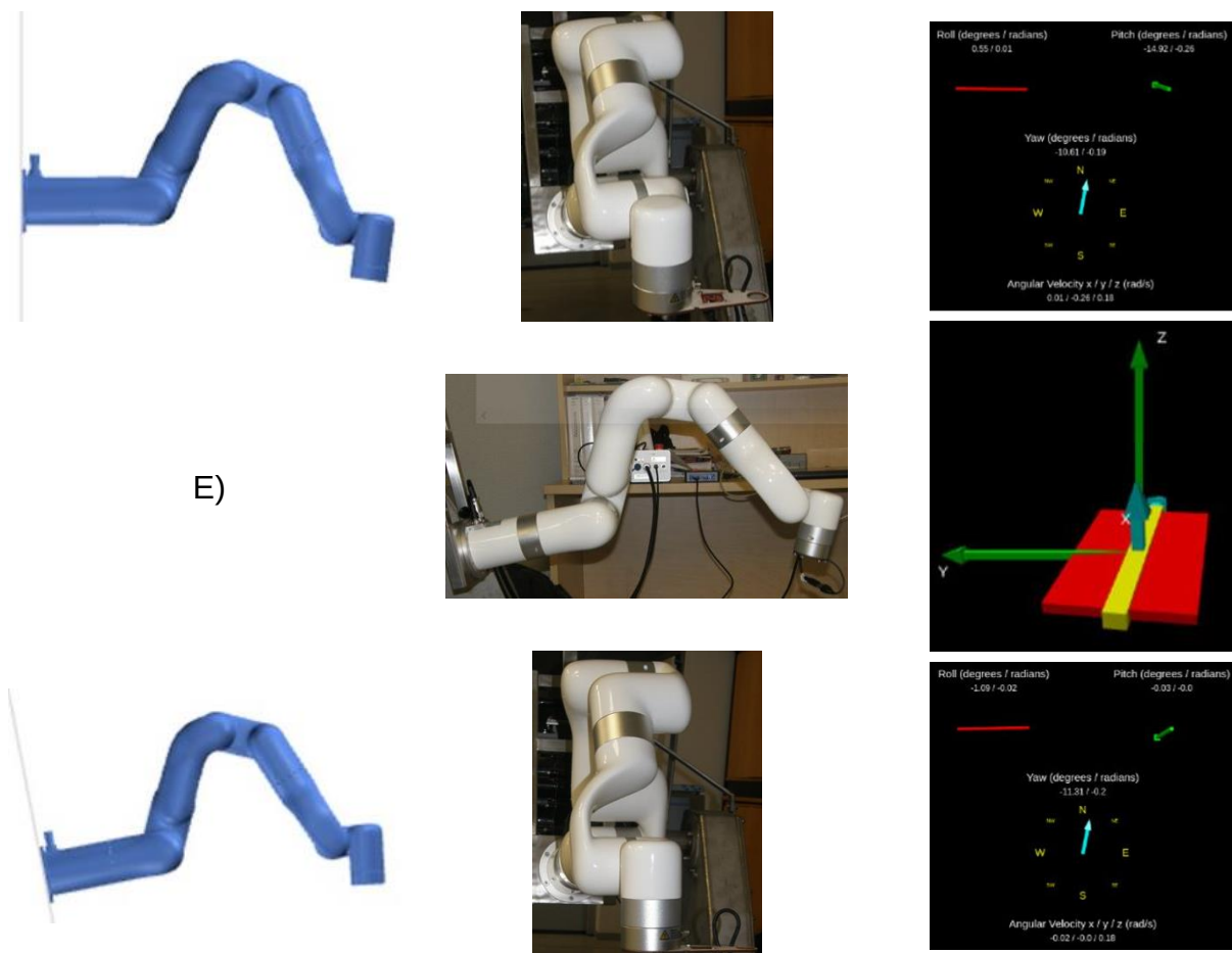
Fig. 3 - Methodology validation results. Beginning state is given in C) roll angle 15 deg and pitch angle 0 deg, E and ending state is given in D). In frames from the left to right xArm base mounting orientation from xArm control GUI, front and side view of actual manipulator state, IMU data visualization razor_imu_9dof razor-pub-and-display.launch.
