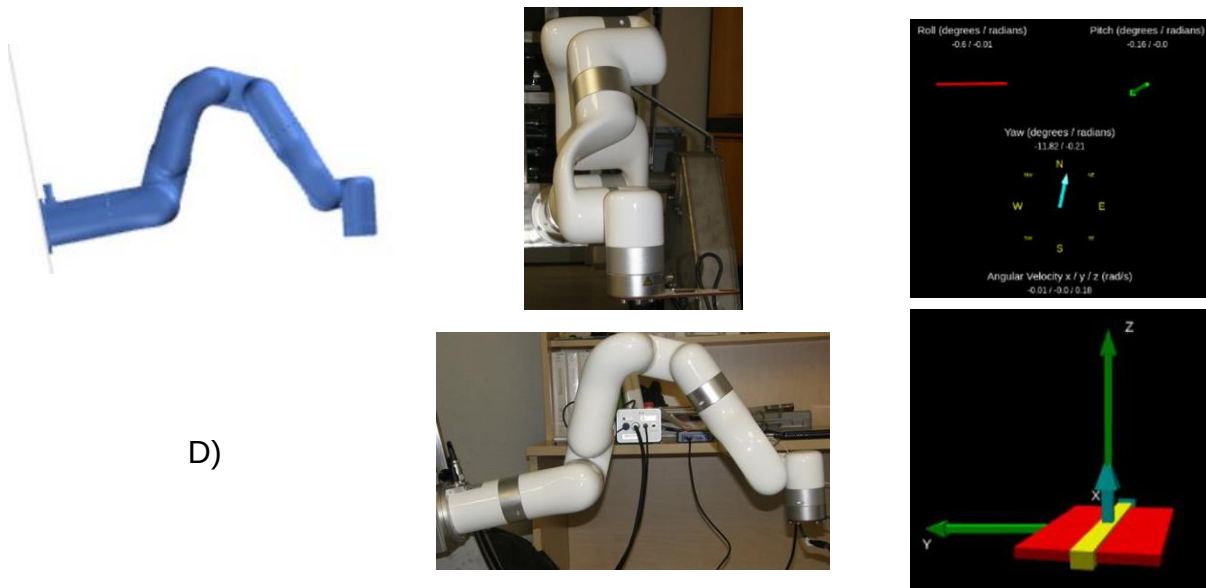
Fig. 3 - Methodology validation results. Beginning state is given in C) roll angle 15 deg and pitch angle 0 deg, E and ending state is given in D). In frames from the left to right xArm base mounting orientation from xArm control GUI, front and side view of actual manipulator state, IMU data visualization razor_imu_9dof razor-pub-and-display.launch.
